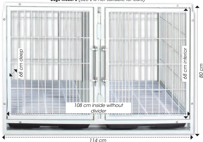
Cage model L (size L is not suitable for cats)
