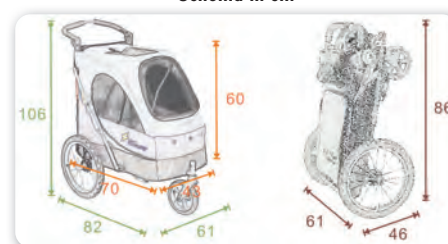
Schema in cm
